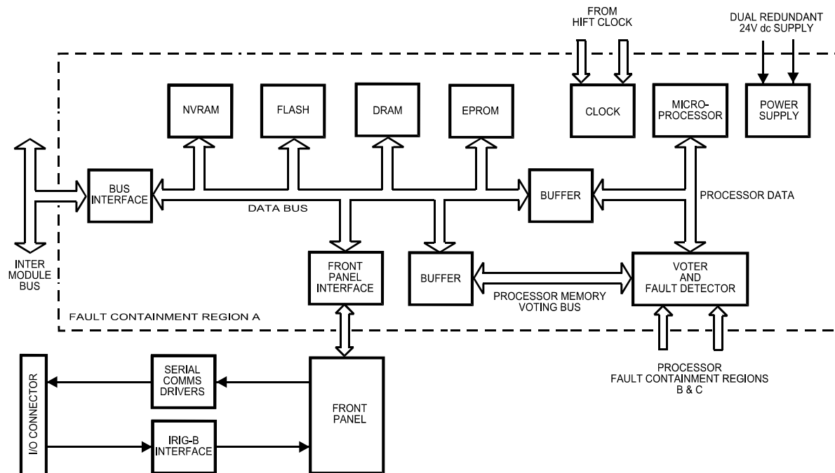
Figure 1 Module Architecture
